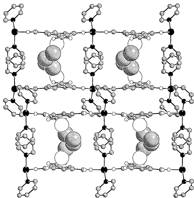
Figure 3. View of the solid-state structure of \text{Zn}(\text{HBTC})(\text{NC}_5\text{H}_5)_2 \cdot \text{C}_2\text{H}_5\text{OH} along the c -axis. The zinc carboxylate layers with the pyridine ligands are shown as sphere-and-stick representation: Zn, large dark; N, small dark; C, small shaded; O, small open. The ethanol guest molecules are shown in the space-filling van der Waals radii with C and O atoms drawn as large shaded and open spheres, respectively. The hydrogen atoms have been omitted for clarity.
